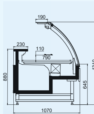
SAPHIRE QUARTZ
